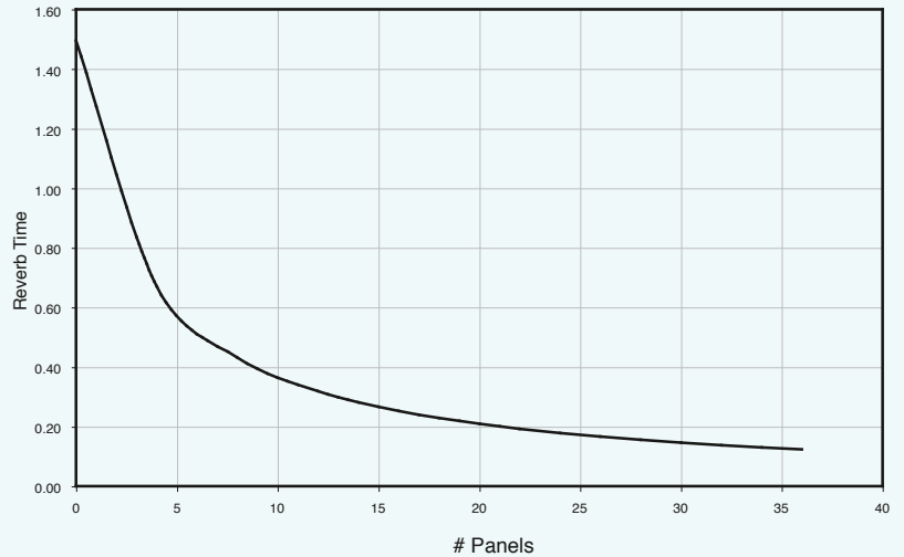
Coverage vs. Reverb Time
